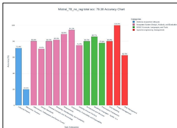
Figure 4. The Accuracy of Mistral 7B without using the RAG infrastructure
