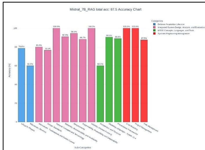
Figure 5. The Accuracy level of Mistral 7B using the RAG infrastructure
