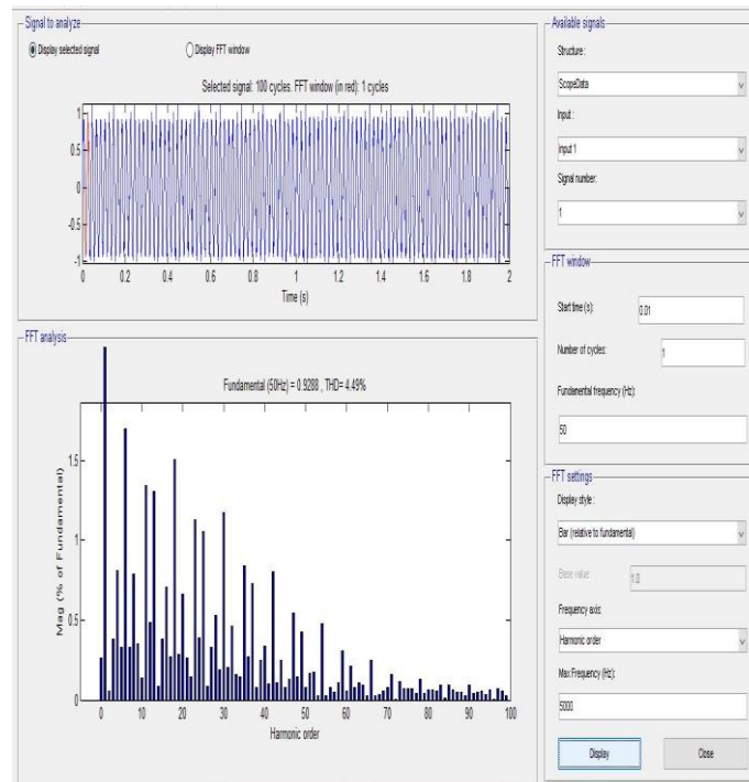
Fig 13- THD value of grid voltage connected WECS with STATCOM
