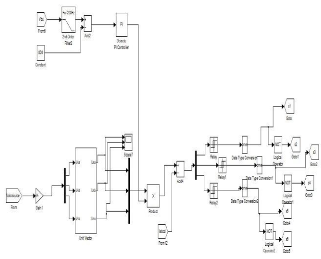
Fig 5- VSC control subsystem for STATCOM
