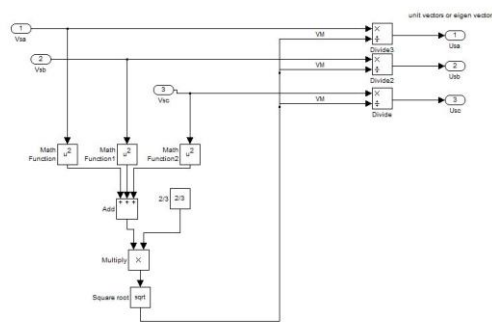
Fig 7- Unit Vector Controlling subsystem
