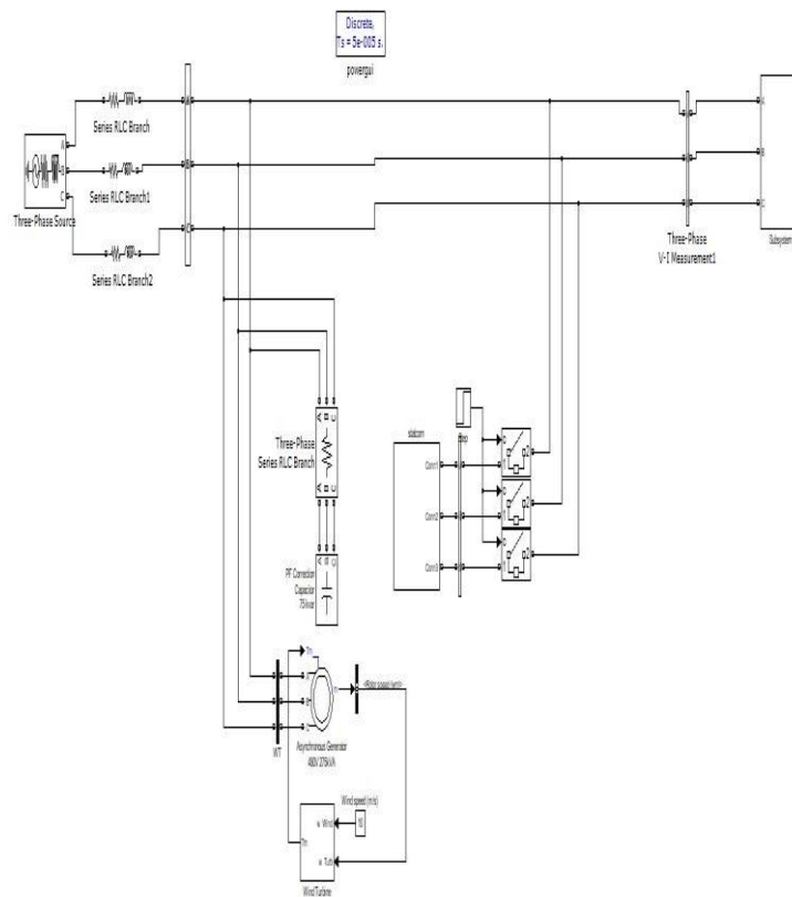
Fig 4- Complete model of grid connected wind system using STATCOM
