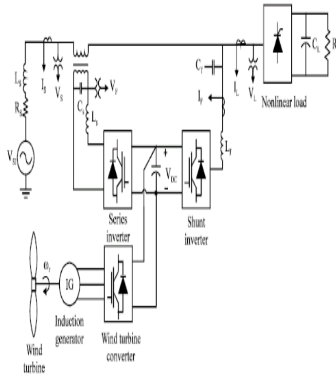
Figure 3 UPQC with Wind Power System
