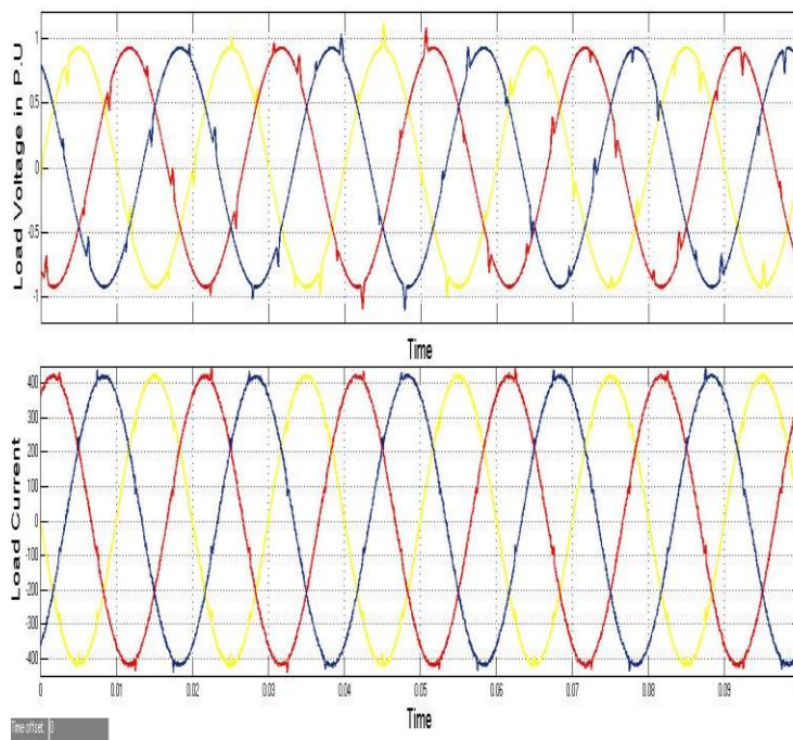
Fig 12- Load side output voltage and current using STATCOM
