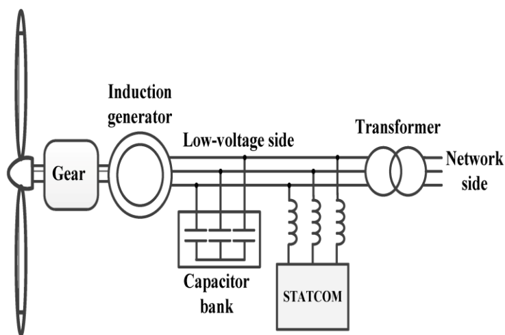
Figure 2 STATCOM with Wind Power System
