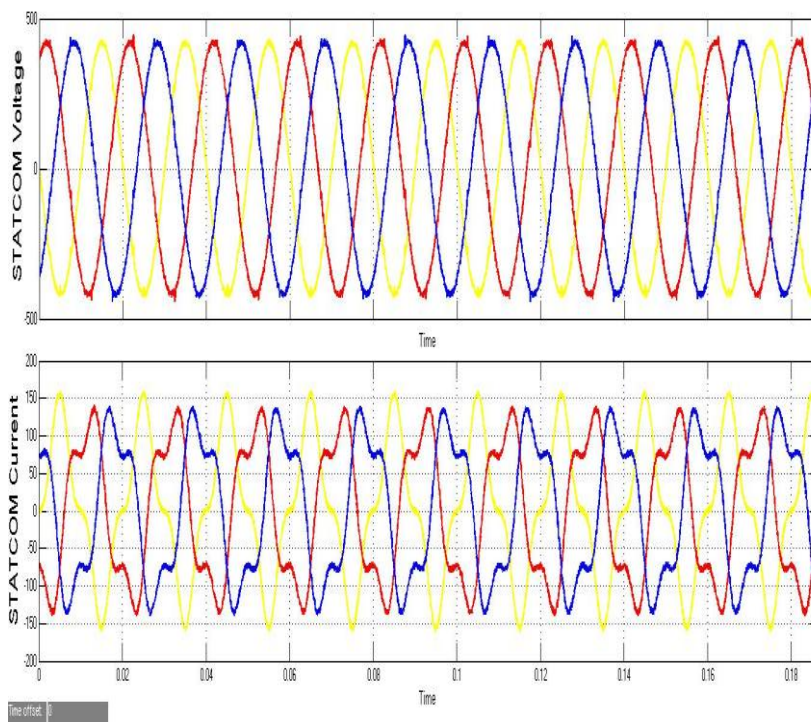
Fig 10- STATCOM controlled voltage and current
