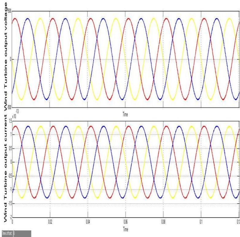
Fig 9- Wind output voltage and Current
