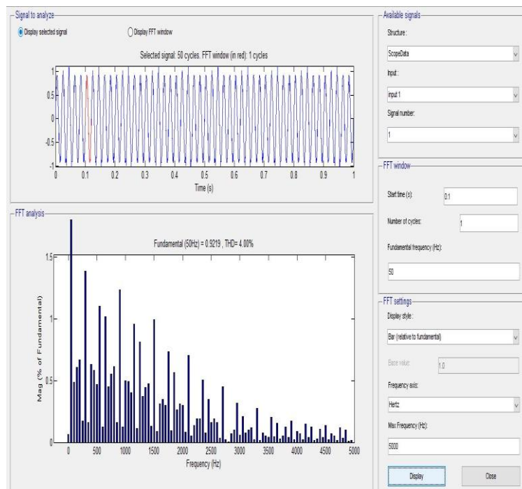
Fig 14- THD value of grid Current connected WECS with STATCOM
