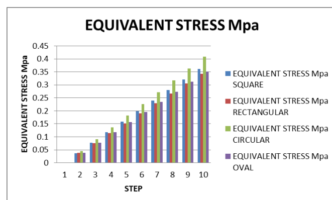
Graph 3 Equivalent Stress
