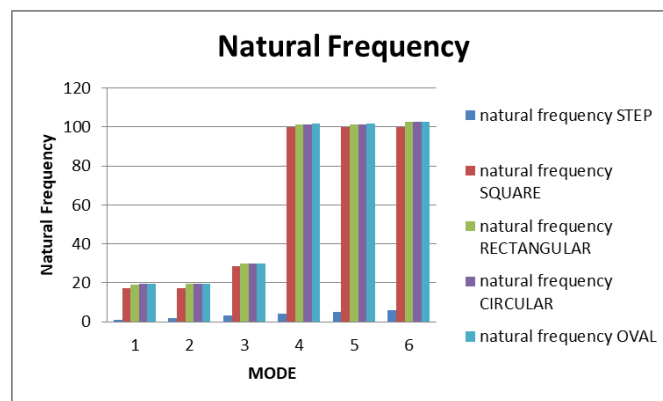
Graph 1 Natural Frequency
