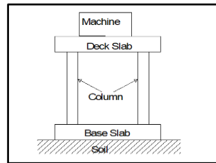
Fig 1 Typical Frame type Foundation
