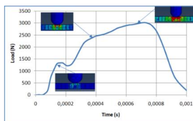
Figure 20: Numerical crushing behavior of an aluminum honeycomb panel with d=6.4 mm.
