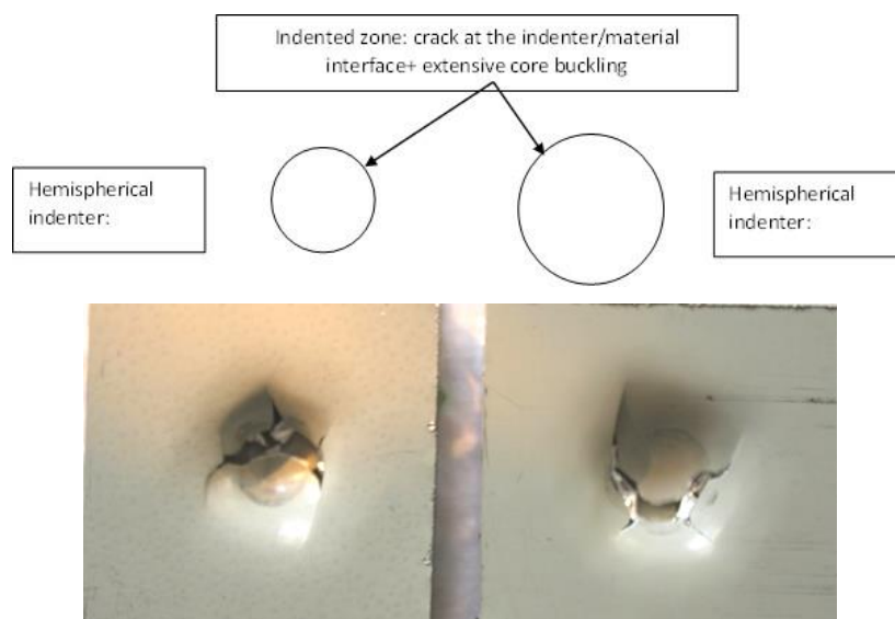
Figure 10: Obtained Failures Modes for an aluminum honeycomb sandwich with cell size of 9.6mm.
