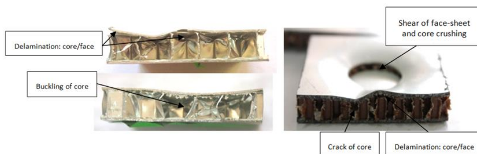
Figure 16: Obtained failures modes.
