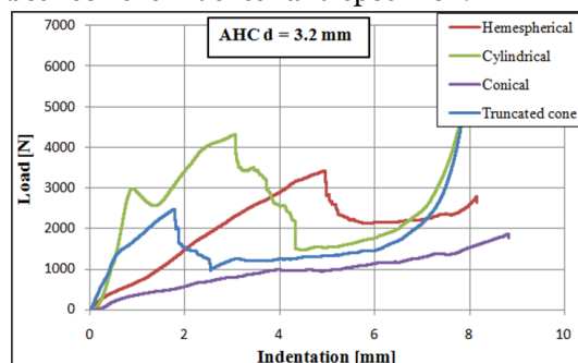
Figure 7: Effect of indenter geometry on indentation behavior (AHC d = 3.2 mm).
