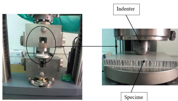
Figure 5: Quasi-Static experiment machine.
