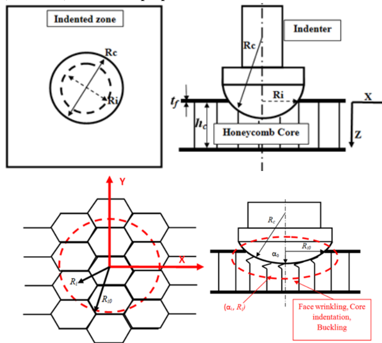
Figure1: Parameters and geometrical configuration of indentation problem.
