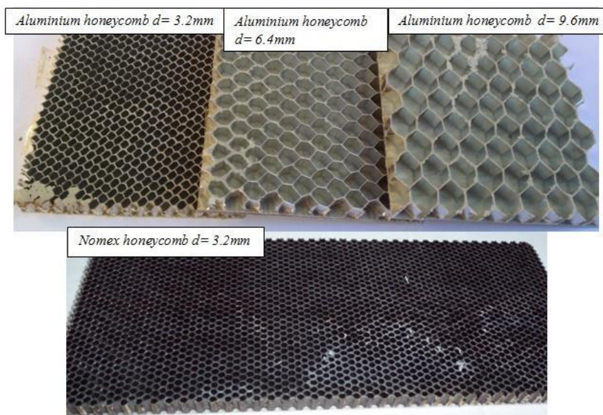
Figure 3: Typologies of investigated sandwiches.
