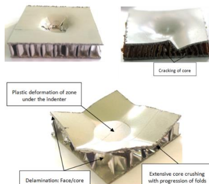
Figure 17: typical failure modes observed during indentation: core crushing and failure of face.
