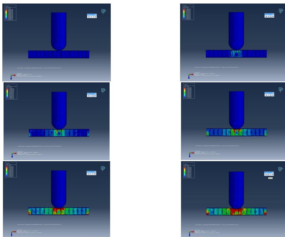
Figure 22: Detailed numerical damage shape at different indenter displacements (AHC d=6.4 )
