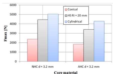
Figure 15: Max indentation load at varying core material for each indenter.
