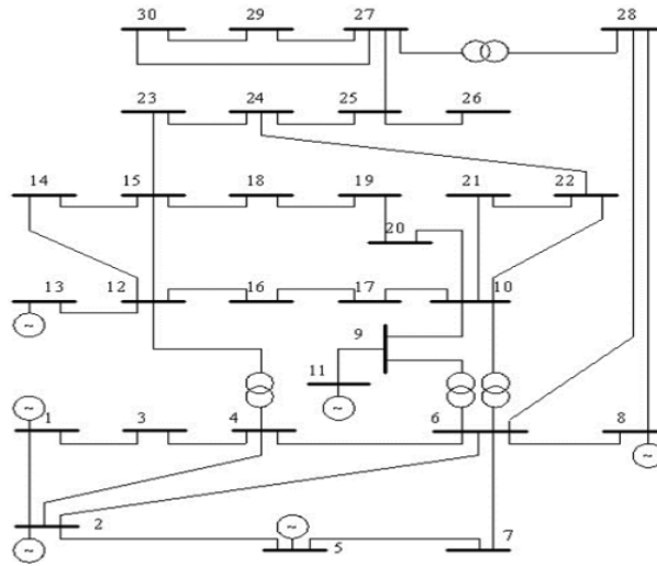
Figure 10. IEEE 30 Bus system Line Diagram
