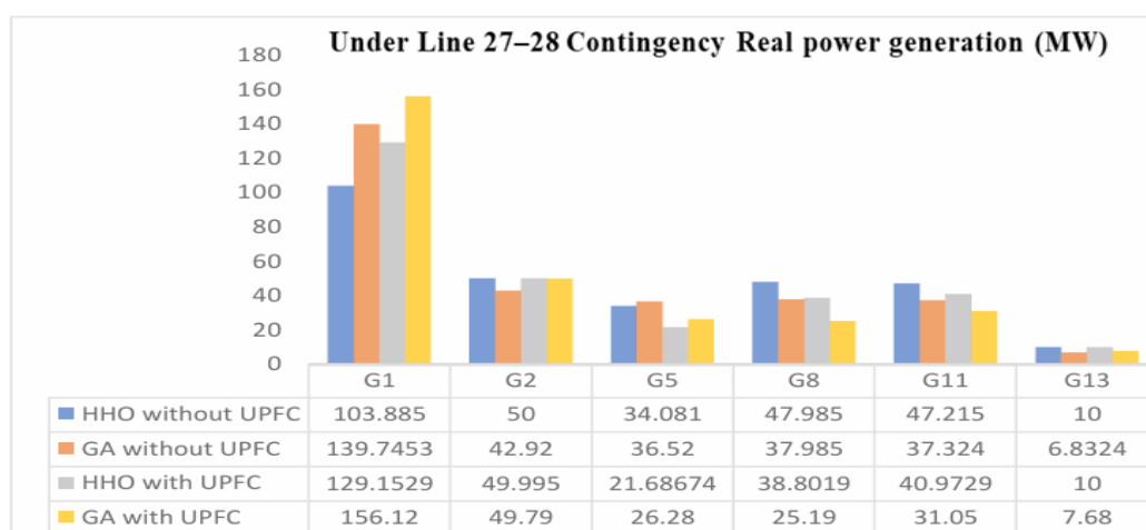
Figure 6. Real Power Generation under Contingency Conditions
