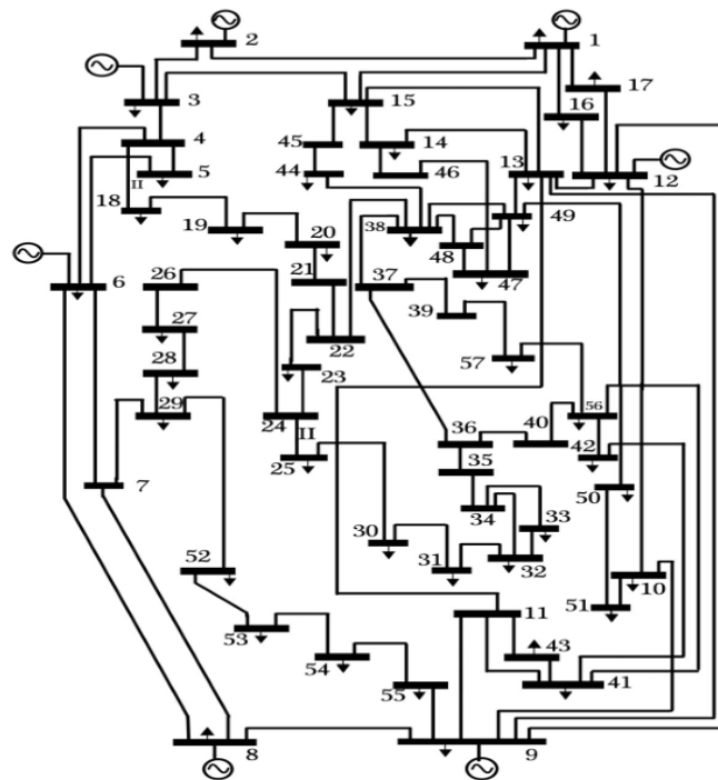
Figure 11. IEEE 57 Bus system Line Diagram
