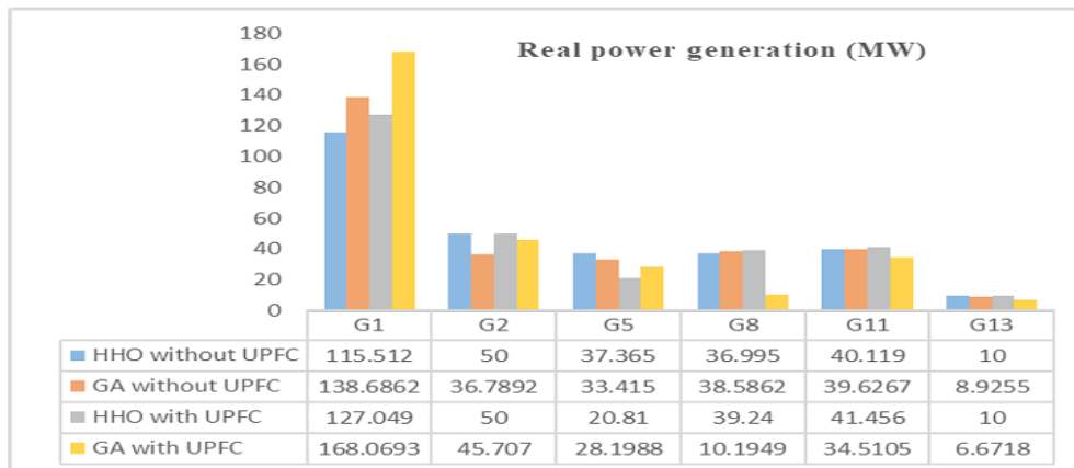
Figure 4. Generator output values with and without UPFC integration in the IEEE 30-bus system under normal operating conditions (no contingency).
