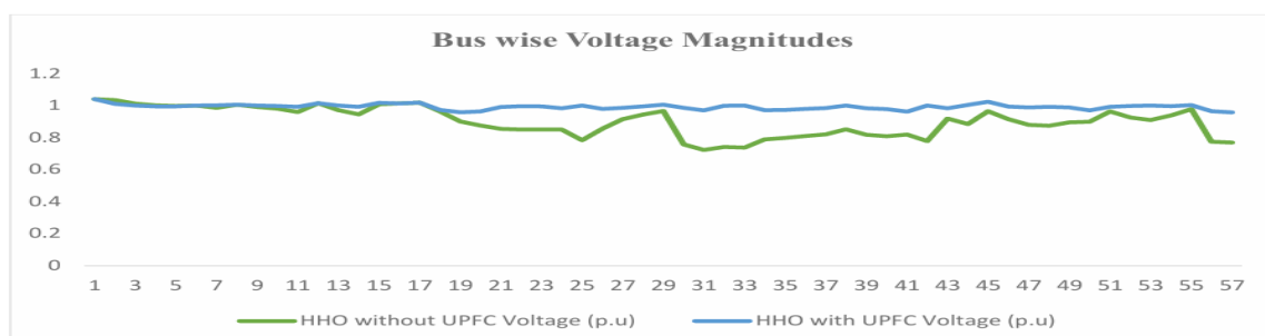
Figure 9. Voltage magnitude profile of the IEEE 57-bus system under contingency conditions with UPFC
