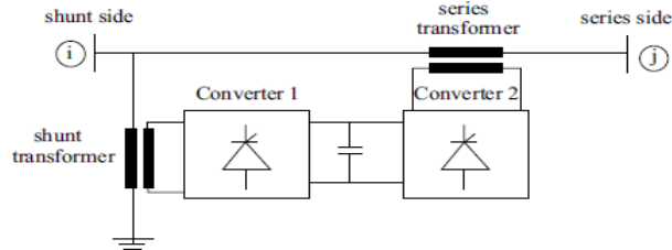
Figure.1. Schematic arrangement of the UPFC
